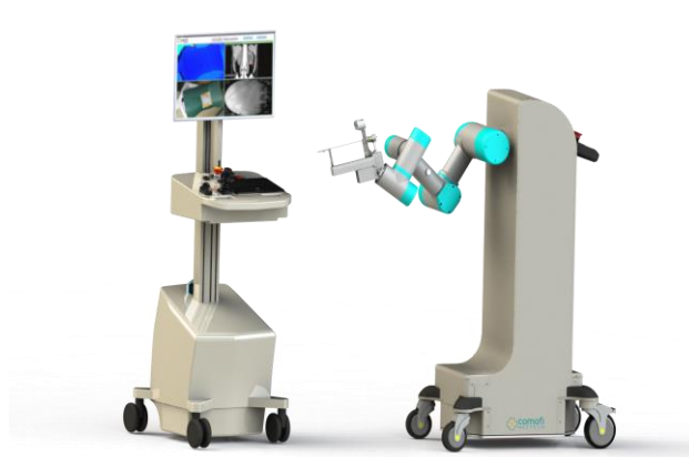
Robot Surgical Intervention: nGuide-PCNL
