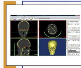
Materialise Mimics
