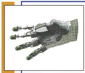
Solidworks 2022
